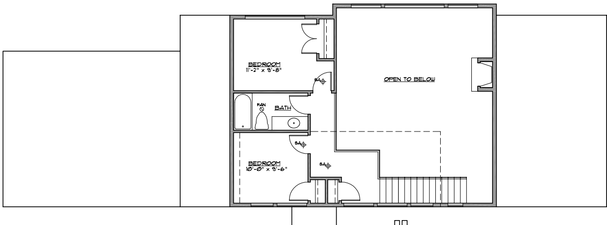
UPPER FLOOR AREA: 460 SQ. FT.
